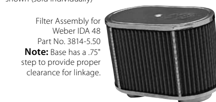
Filter Assembly for Weber IDA 48 Part No. 3814-5.50
